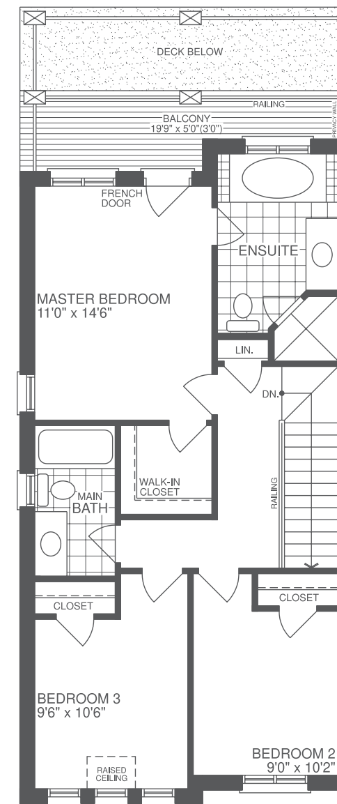
SECOND FLOOR ELEVATION A 2056 sf
