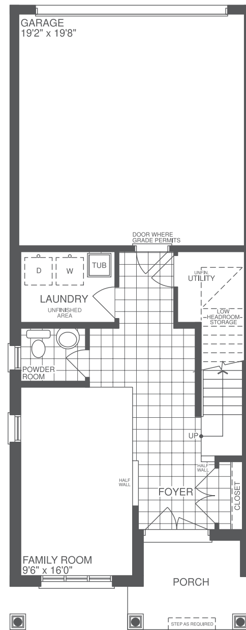
GROUND FLOOR ELEVATION A 2056 sf
